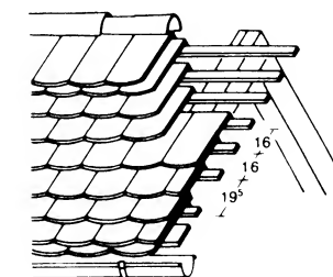
14 Double roof (plain tiles) heavy roofing, 0.6 kN/m 2 , 34-44 tiles/m 2
